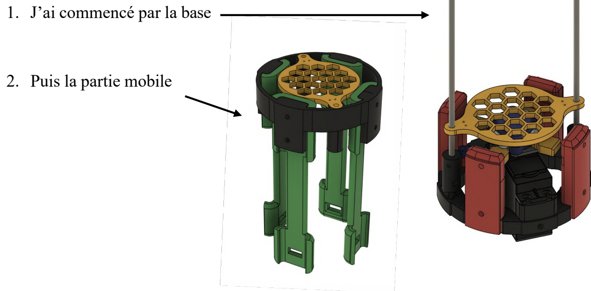
Figure 10 : Assemblage final.
